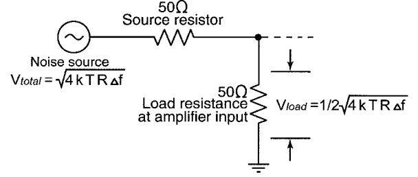
Fig. 7. Equivalent input circuit showing the thermal noise generator with a source resistance of 50 \Omega and terminated into the amplifier’s input (load) resistance, which is also 50 \Omega . Note that the thermal noise voltage is divided in half at the amplifier’s input.
